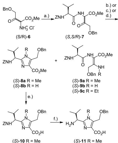
Scheme 1. Reagents and conditions: (a) Z -( S )-Val-OH, i BuOCOC 2 Cl, NMM, DCM, –50 °C, 65%; (b) TFA, MeNH 2 /EtOH, xylene, Δ, 69% for 8a ; (c) TFA, NH 3 /MeOH, xylene, Δ, 75% (mixture of 8b and 9b ); (d) TFA, EtNH 2 /H 2 O, xylene, Δ, 70% for 9c ; (e) aq NaOH, MeOH, dioxane, 20 °C then aq HCl, 99%; (f) 1,4-cyclohexadiene, EtOH, Pd(OH) 2 /C, 20 °C, 97%.
