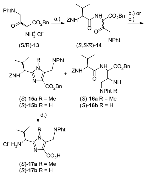
Scheme 3. Reagents and conditions: (a) Z-(S)-Val-OH, i BuOCOC 2 Cl, NMM, DCM, –30 °C, 88%; (b) TFA, MeNH 2 /EtOH, xylene, Δ, 63% for 15a and 7% for 16a ; (c) TFA, NH 3 /MeOH, xylene, Δ, 34% for 15b and 44% for 16b ; (d) H 2 , Pd/C, MeOH, aq HCl, 99% for 17a , 99% for 17b .
