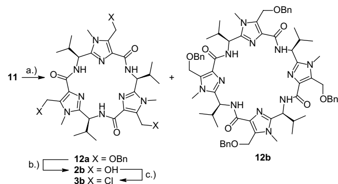
Scheme 2. Reagents and conditions: (a) PyBOP, i Pr 2 NEt, DMF, 20 °C, 21% for 12a and 9% for 12b ; (b) H 2 , Pd/C, DCM, 97%; (c) SOCl 2 , CHCl 3 , Δ, 99%.
