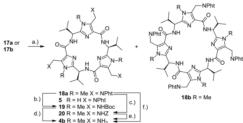
Scheme 4. Reagents and conditions: (a) PyBOP, i Pr 2 NEt, DMF, 20 °C, 51% for 18a and 8% for 18b (starting from 17a ); 40% for 5 (starting from 17b ); (b) N 2 H 4 ·H 2 O, THF/DCM/EtOH then Boc 2 O, 20 °C, 97%; (c) (1) N 2 H 4 ·H 2 O, THF/DCM/EtOH, 20 °C, (2) ZCl, Et 3 N, DCM, 20 °C, 77%; (d) HCl/EtOAc, 20 °C, 99%; (e) H 2 , Pd/C, aq HCl, MeOH, 88%; (f) N 2 H 4 ·H 2 O, THF/DCM/EtOH, 20 °C then acidic work-up, 74%.
