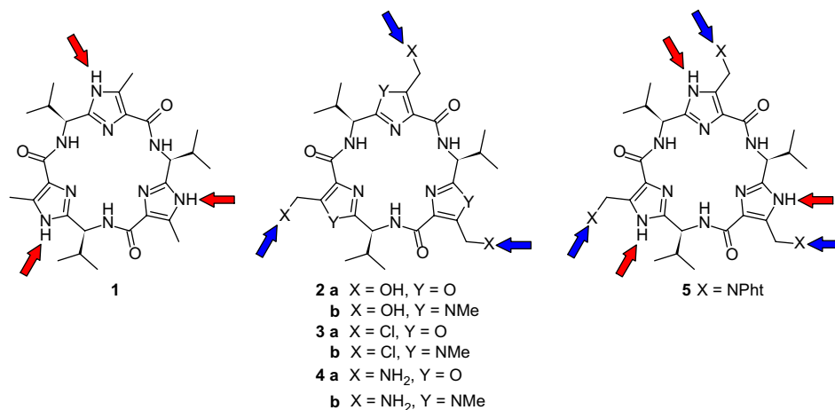
Figure 1. Structural formula of chiral macrocyclic scaffolds with three or six anchoring sites.
