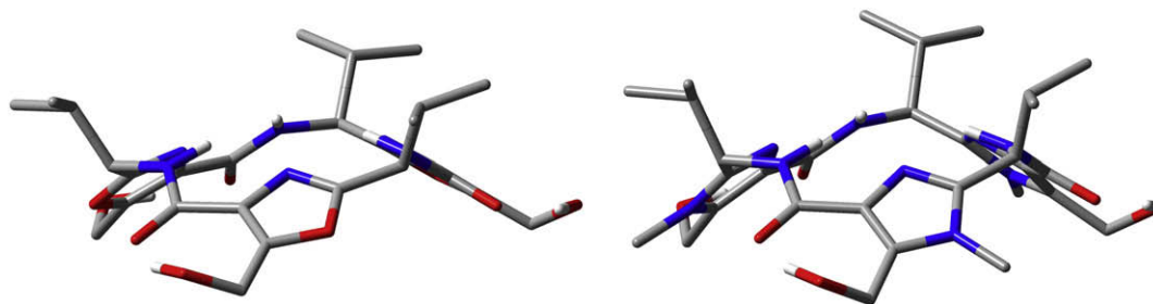
Figure 2. Molecular structures of the energetically preferred conformers of 2a and 2b calculated using B3LYP/6-31G*; all non-polar hydrogen atoms have been omitted for clarity.
